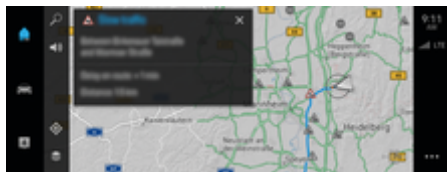
Fig. 15 Risk Radar
